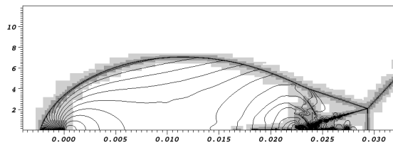
Cartesian base grid 360 \times 160 cells on domain of 36 \text{ mm} \times 16 \text{ mm} with up to 3 refinement levels with r_l = 2, 4, 4 and \Delta x_{1,2} = 3.125 \mu\text{m} , 38 h CPU
