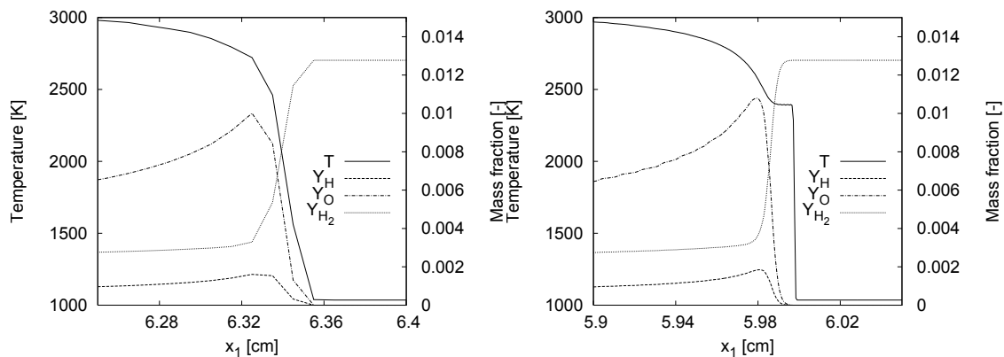
Approximation of H_2 : O_2 detonation at \sim 1.5 P_{ts}/l_{ig} (left) and \sim 24 P_{ts}/l_{ig} (right)
