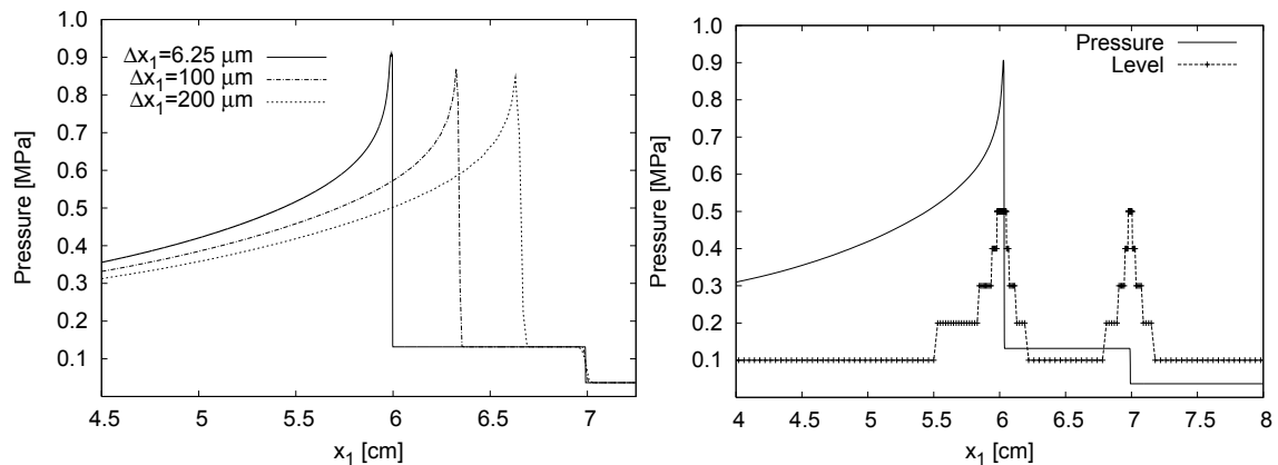
Left: Comparison of pressure distribution t = 170 \mu s after shock reflection. Right: Domains of refinement levels
