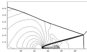
\Delta x = 12.5 mm
