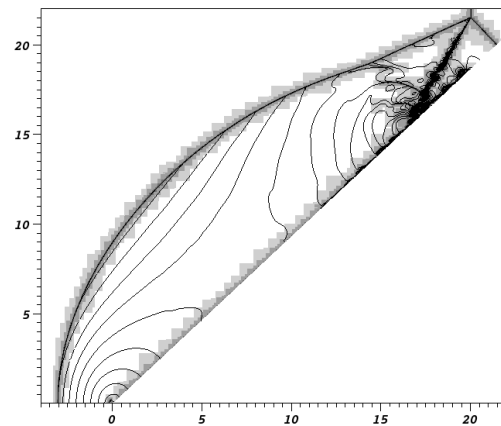
GFM base grid 390 \times 330 cells on domain of 26 \text{ mm} \times 22 \text{ mm} with up to 3 refinement levels with r_l = 2, 4, 4 and \Delta x_{e,1,2} = 2.849 \mu\text{m} , 200 h CPU
